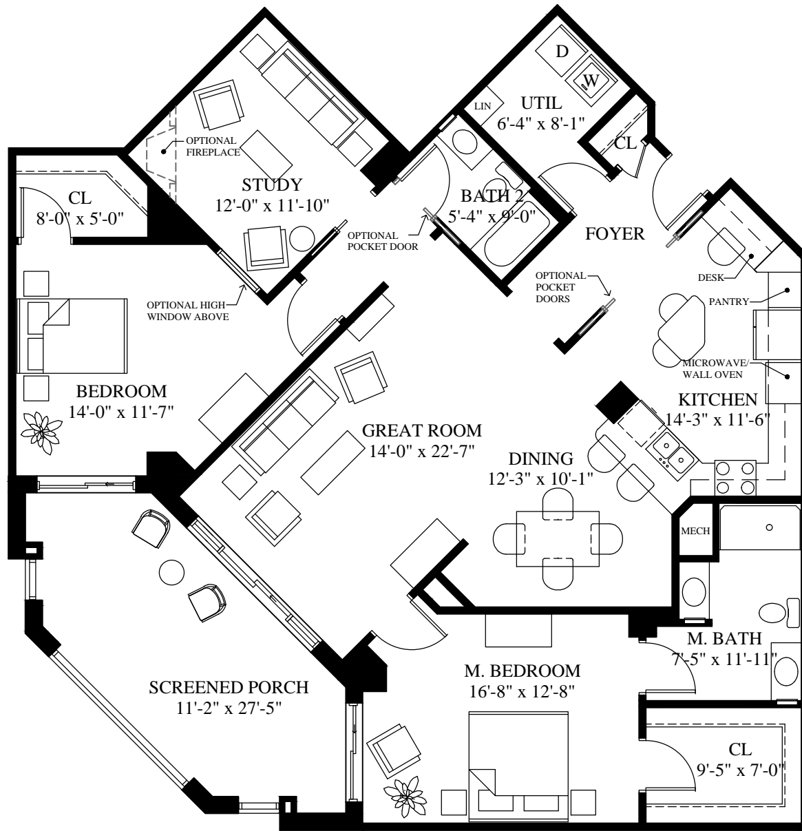
UNIT E FLOOR PLAN 1,739 SQ. FT.
